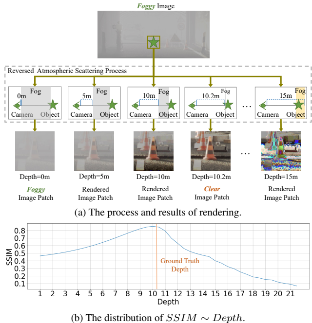
Figure 1. The Visualization of depth hints from fog. (a) We reverse the atmospheric scattering process by removing the fog among different depth ranges. Only the depth near the ground truth leads to a clear image. We deem this observation as the depth hint. (b) We further illustrate the distribution of rendered image quality in depth. We measure the image quality via the structural similarity (SSIM) metric. We find that the closer the depth candidate is to the ground truth, the better the rendered image quality is.
